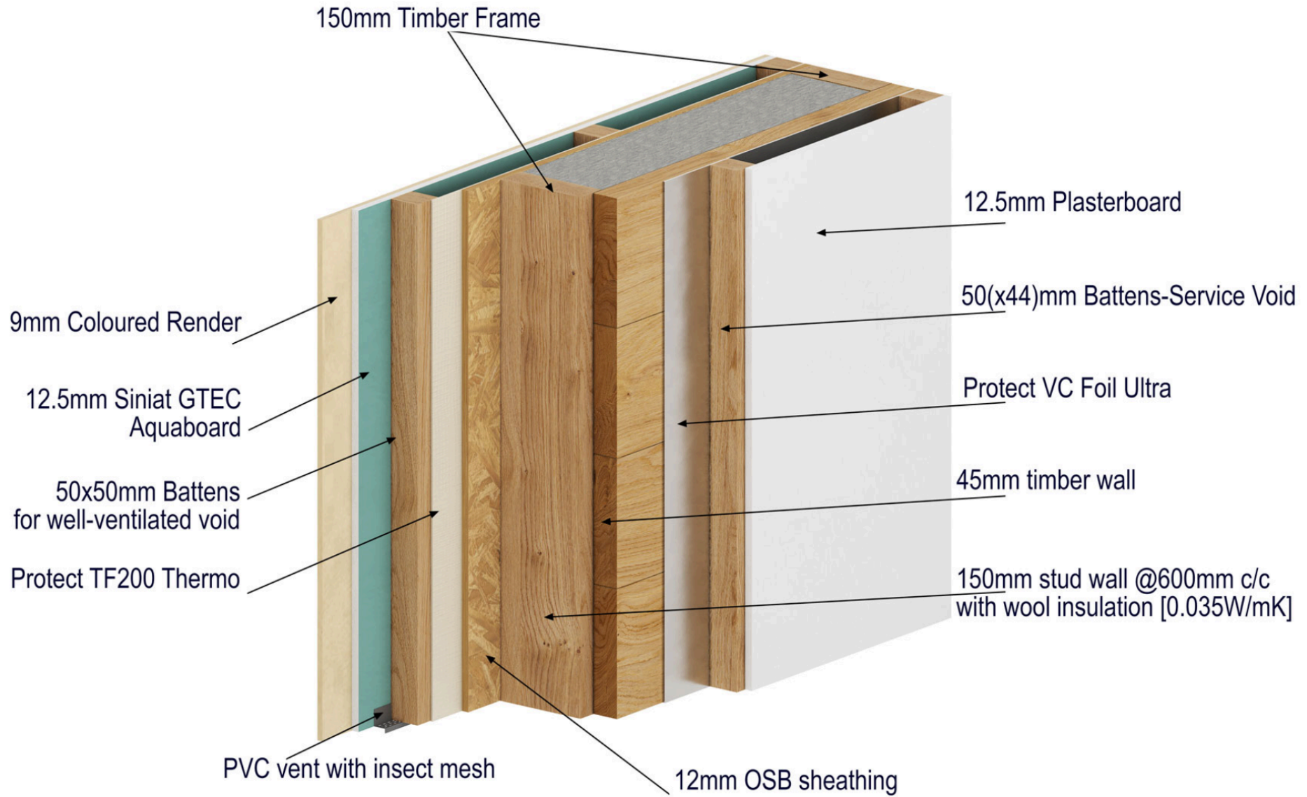
Details of construction of A2 Timber Frame Wall
