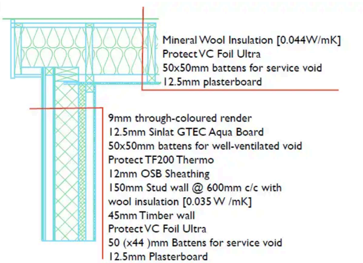
Timber Frame Walls & Roof Verge
